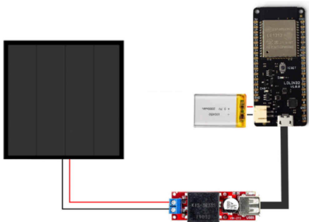
Figure 46: Connections between solar panel, DC-DC converter, ESP32 and battery
